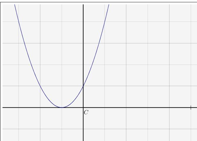
Figure 2 : p_1 = x^2 + 2x + 1
