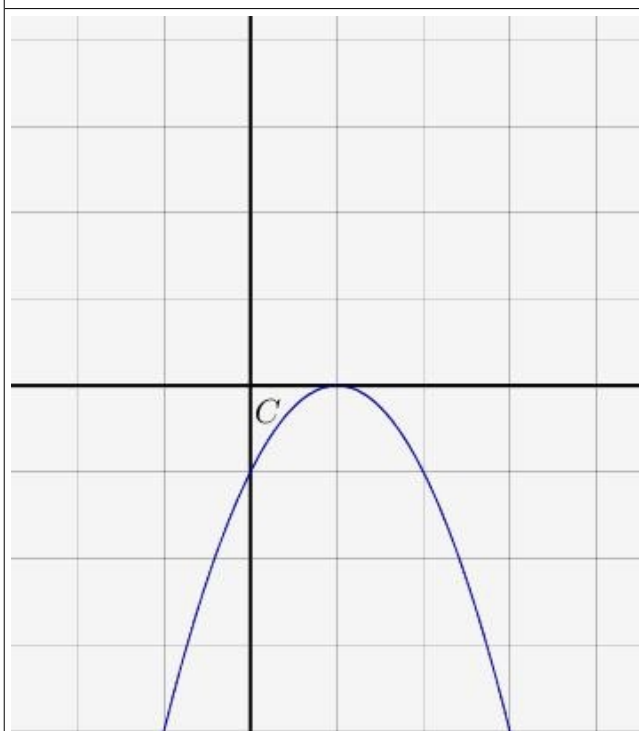
Figure 5 : p_4 = -x^2 + 2x - 1
