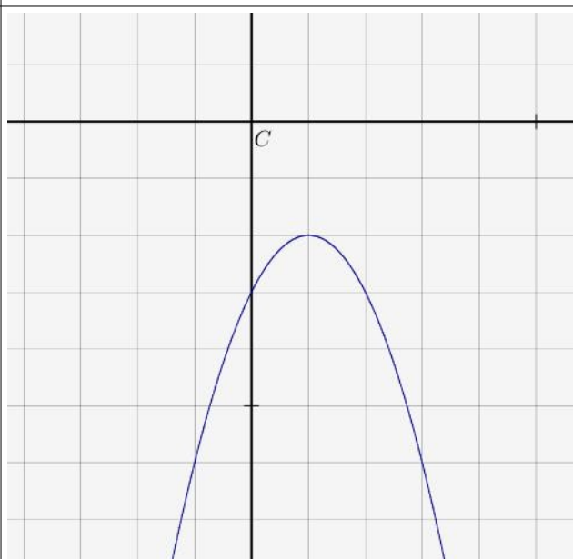
Figure 4 : p_3 = -x^2 + 2x - 3
