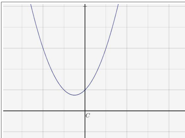
Figure 1 : p_6 = x^2 + x + 1
