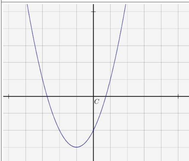
Figure 3 : p_5 = x^2 + 2x - 2
