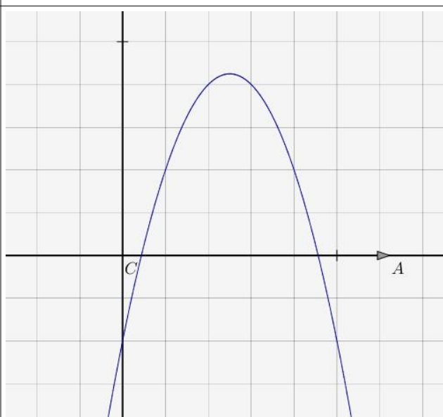
Figure 6 : p_2 = -x^2 + 5x - 2
